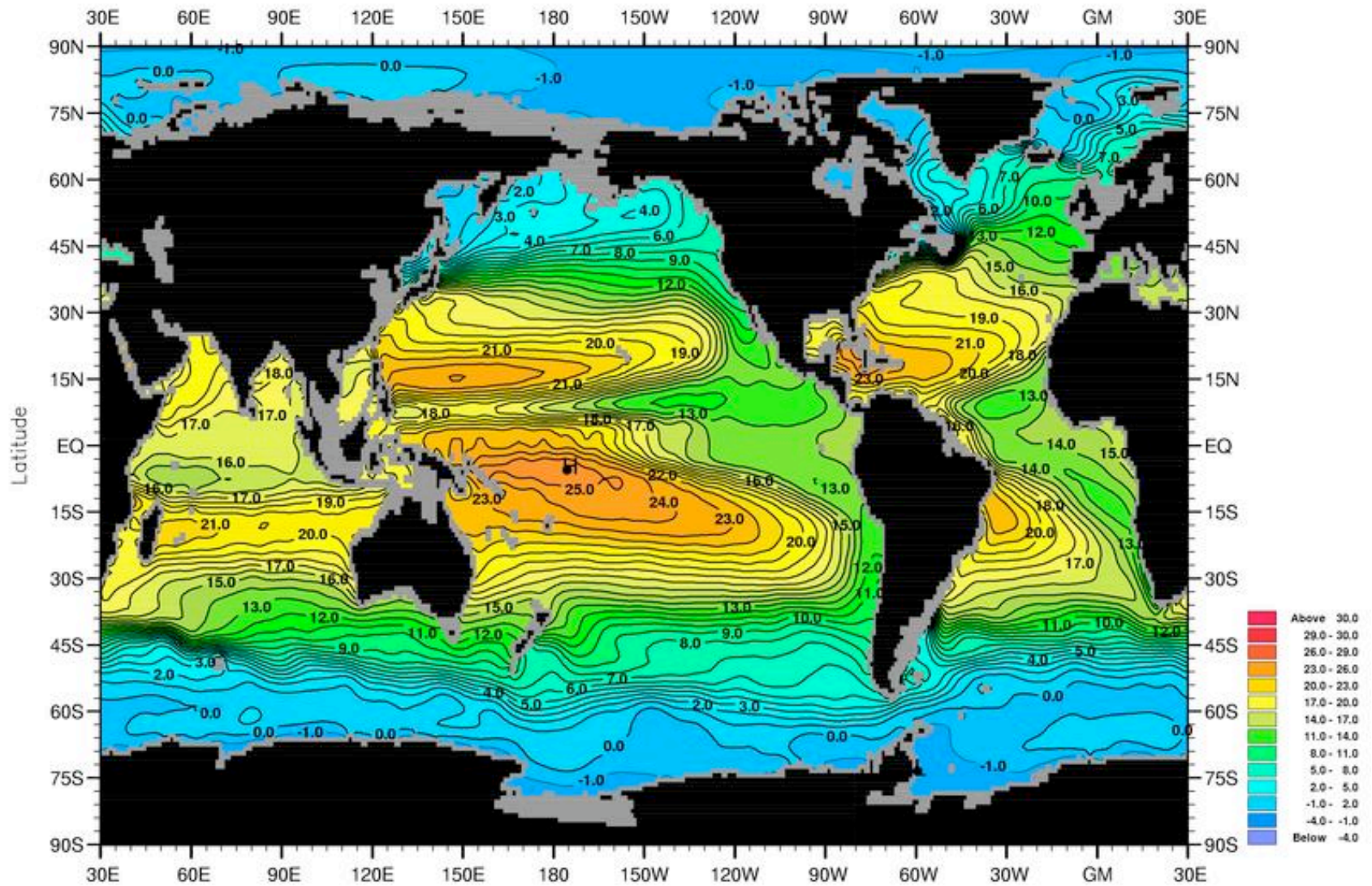
Figure 4: Map of pressure at 150 meter depth in the ocean
